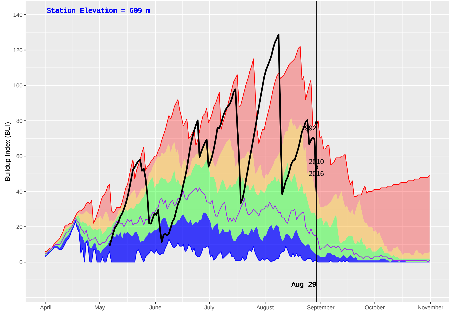
BOB QUINN LAKE (113) : Historical (1984–2016) and Current (2018) Daily Buildup Index (BUI)
